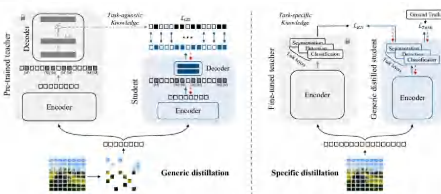
Figure 2. Diagram of the proposed generic-to-specific distillation (G2SD). [M] denotes mask token. In the generic distillation stage ( left ), masked images are converted to patches and fed to both the teacher and student encoders for feature extraction. Feature predictions of the student decoder are aligned with those of the teacher at both visible and predicted patches. In the specific distillation stage ( right ), student models are trained to have consistent predictions with teacher models fine-tuned on the specific task.
