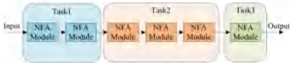
Figure 2: The illustration of an adaptive training framework based on NFA for cascaded multi-task training.
