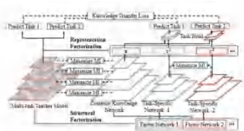
Fig. 2: The overall framework of the proposed knowledge factorization. The factor networks are trained to mimic the prediction of the teacher. The CKN learns to maximize the mutual information between input and its features, whereas the TSNs are dedicated to minimizing the task-wise mutual information.
