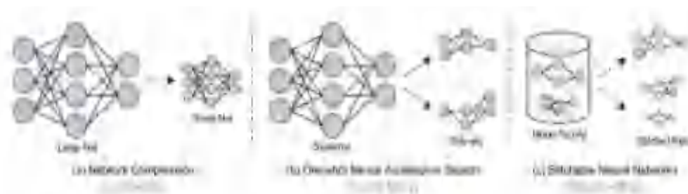
Figure 1. Comparison with previous scalable deep learning frameworks. (a) Network compression shrinks a large network into a smaller one by techniques such as pruning, quantization and knowledge distillation, etc., which is a time-consuming mapping. (b) One-shot neural architecture search first trains a generator that supports diverse architectural settings and then specializes on search given the target accuracy constraint during deployment, which is a case of one-to-many. (c) Our proposed stitchable Neural Network directly stitches the all-the-kind family of pre-trained models and quickly obtains new networks of different model design and deployment (a novel many-to-many paradigm).
