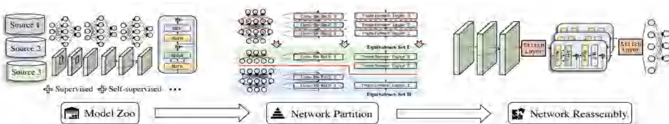
Figure 1: Overall workflow of DeRy. It partitions pre-trained models into equivalent sets of neural blocks and then reassemble them for downstream transfer. Both steps are optimized through solving constrained programs.
